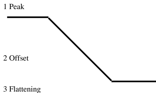
Figure 1. The shape of age effects on SLT.
